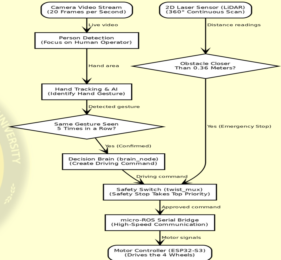
Figure 3.1: Dataflow Pipeline from Sensor Feeds to Wheel Actuation
